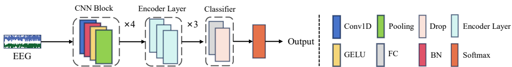
Figure 6: The detailed pre-trained model architecture.
